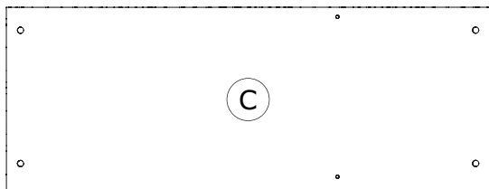
PI7674 1161x443x16mm
