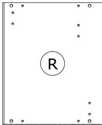
FI9252 350x286x16mm
